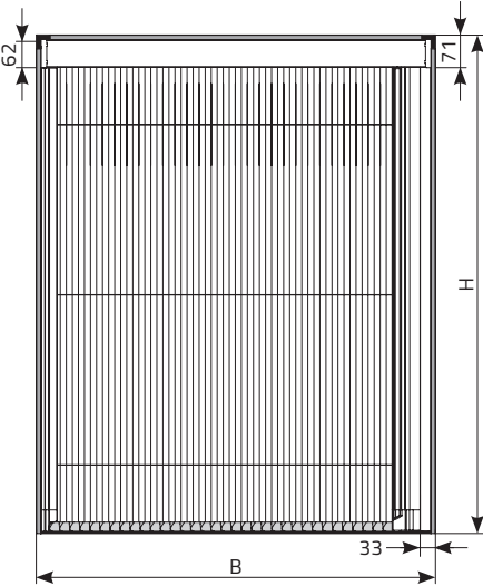
window/facade-mount
