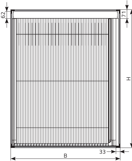
window/facade-mount
