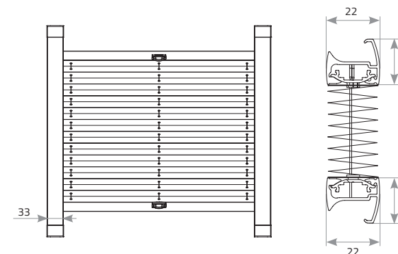
cross-section of the side guide
