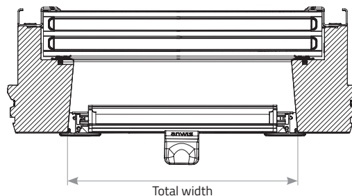
cross-section of the side guide
