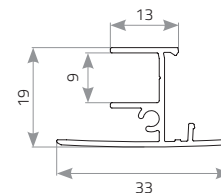
cross-section of the side guide
