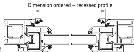
Dimension ordered – recessed profile
