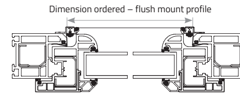
Dimension ordered – flush mount profile
