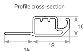
Profile cross-section
