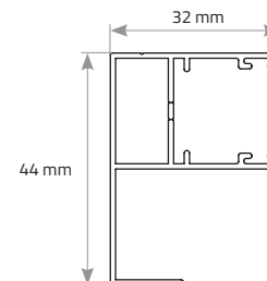
Fig. 3 Side channel with extension
