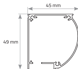
Fig. 1 Cassette cross section
