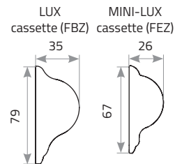
Fig.3 Type of cassette
