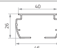
Szyna Górna Aluminiowa A-2006 Aluminium Head Rail A-2006
