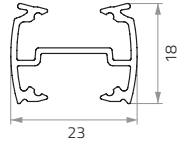
Rail – cross-section
